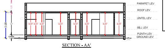
SECTION - AA'
