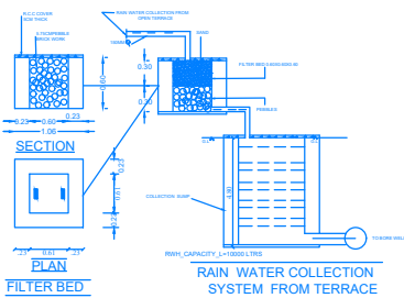
RAIN WATER COLLECTION SYSTEM FROM TERRACE
