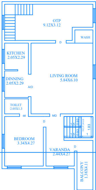
EXI.FIRST FLOOR PLAN
