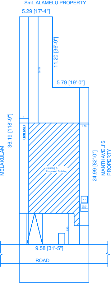
FOUR BOUDIRES ARE AS PER SITE SITE PLAN Scale 1:200
