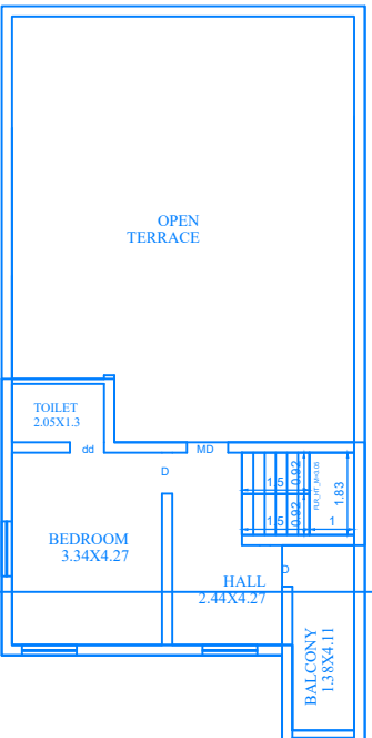
PRO.SECOND FLOOR PLAN
