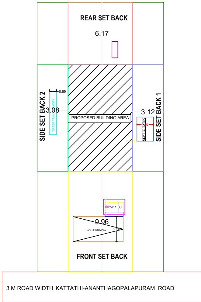
SITE PLAN
