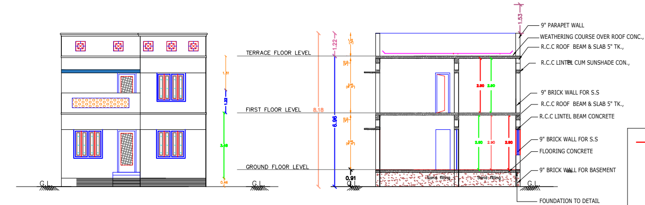
FRONT ELEVATION
