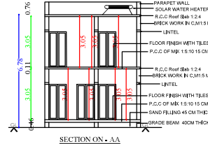
SECTION ON-A-A
