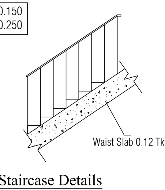
Staircase Details
