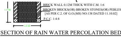
SECTION OF RAIN WATER PERCOLATION BED
