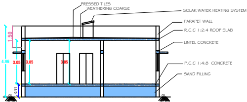
SECTION AT A-A
