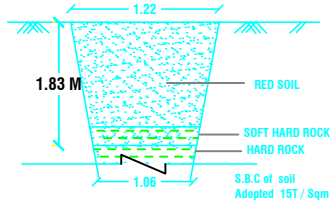
TRIAL PIT DETAILS
