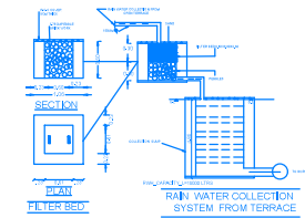
RAIN WATER COLLECTION SYSTEM FROM TERRACE
