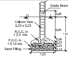
COLUMN DETAILS NOT TO SCALE
