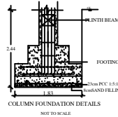
COLUMN FOUNDATION DETAILS
