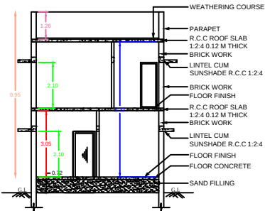
SECTION "N-R"
