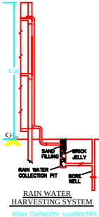
RAIN WATER HARVESTING SYSTEM RWH_CAPACITY_L=1000LTRS
