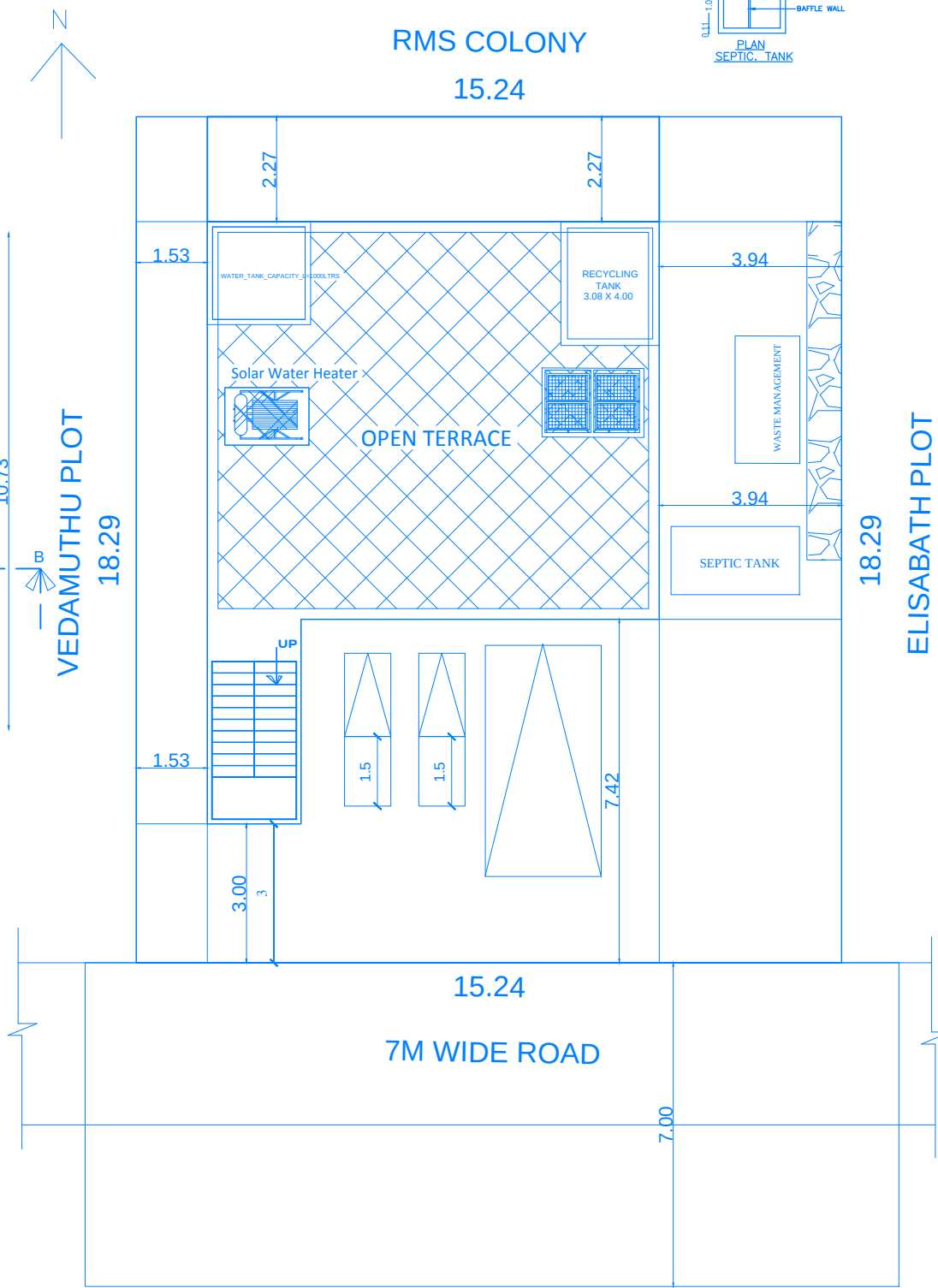
SITE PLAN
