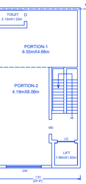
PRO.FIRST FLOOR PLAN
