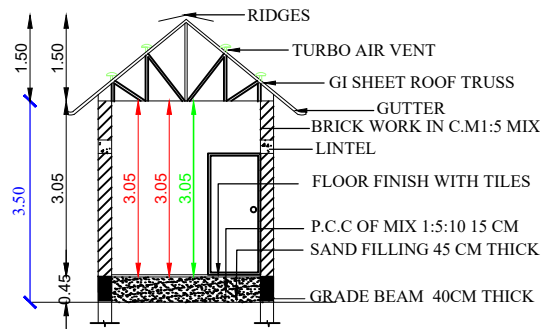
SECTION- AB
