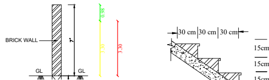
BASE STEPS 1:25
