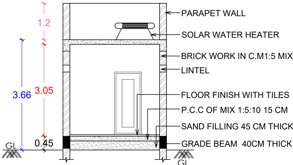
SECTION- AB
