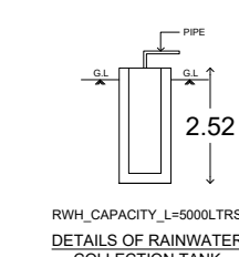
RWH CAPACITY L=5000LTRS DETAILS OF RAINWATER COLLECTION TANK
