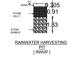
RAINWATER HARVESTING PIT (RWHP)
