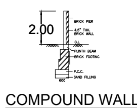
COMPOUND WALL
