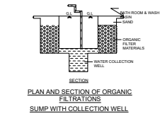
PLAN AND SECTION OF ORGANIC FILTRATION WASTE WATER TREATMENT (NOT TO SCALE)
