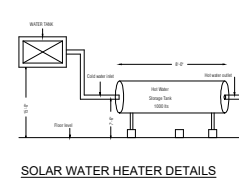
SOLAR WATER HEATER DETAILS (NOT TO SCALE)
