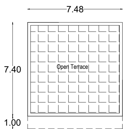
PRO.TERRACE FLOOR PLAN
