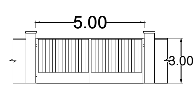
MAIN GATE
