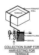
COLLECTION SUMP FOR RAINWATER HARVESTING
