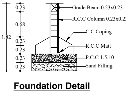
Foundation Detail
