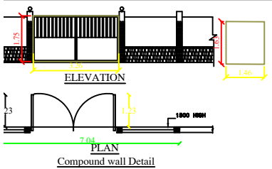
Compound wall Detail
