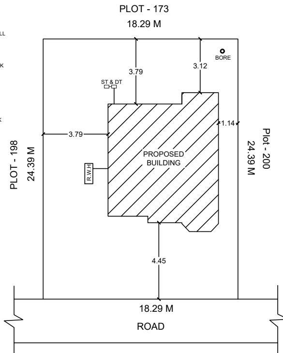
SITE PLAN
