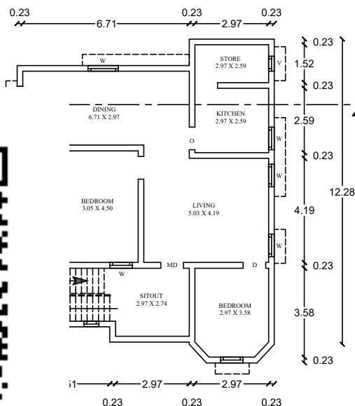
POSED FIRST FLOOR PLAN
