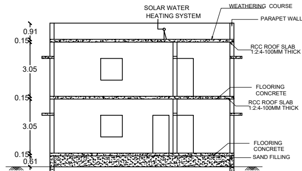
SECTION NP
