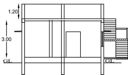
SECTION "A-B"
