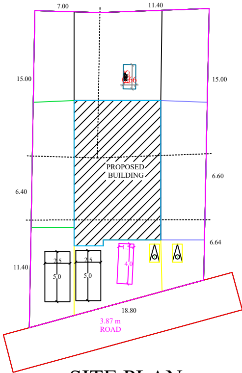
SITE PLAN
