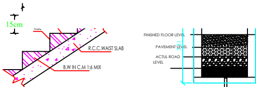
SECTION OF STAIRCASE
