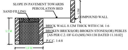
SECTION OF RAIN WATER PERCOLATION BED
