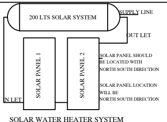
SOLAR WATER HEATER SYSTEM
