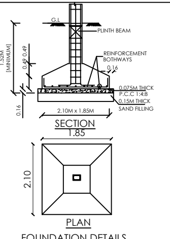
FOUNDATION DETAILS
