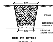
TRIAL PIT DETAILS NOT TO SCALE
