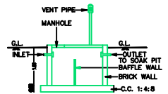
SECTION OF SEP.TANK
