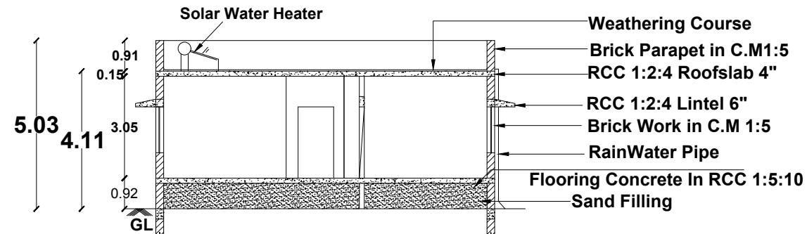
SECTION - "A B"
