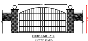
COMPOUND GATE (NOT TO SCALE)
