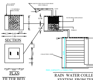
RAIN WATER COLLECTION SYSTEM FROM TERRACE
