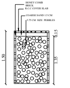
SECTION
