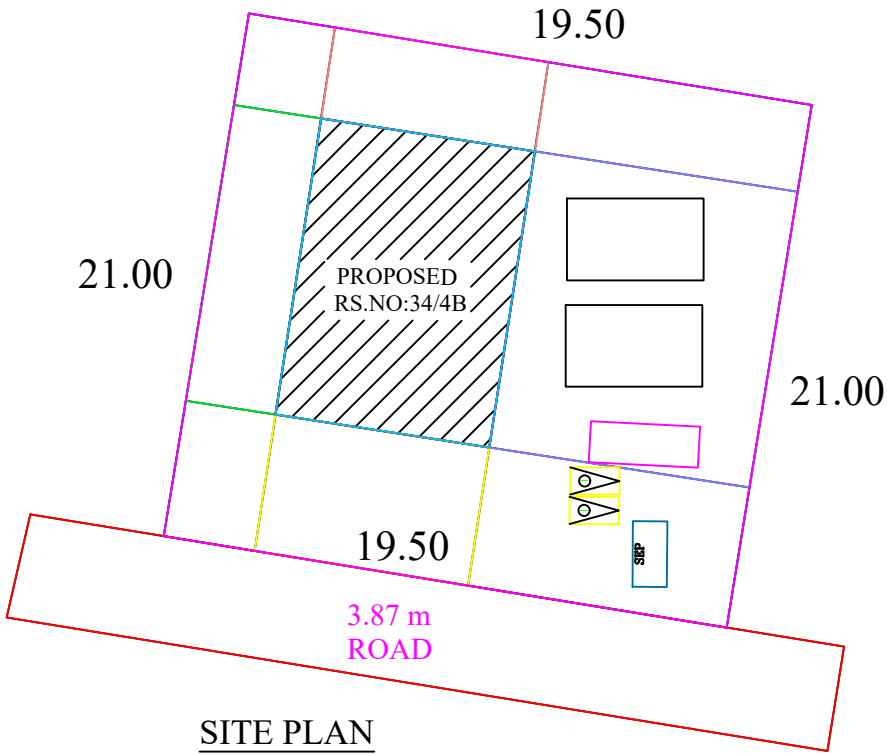
TOPO PLAN
