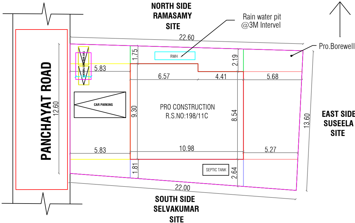
SITE PLAN
