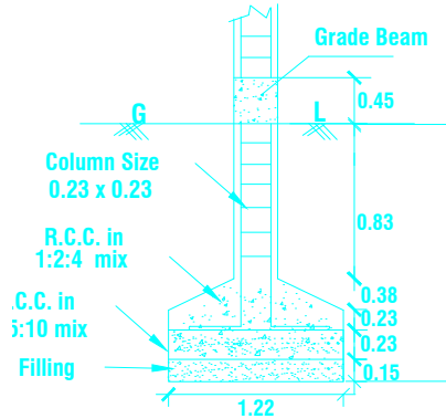
COLUMN DETAILS
