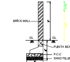
COMPOUND WALL DETAIL
