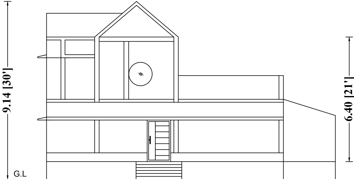
FRONT ELEVATION
