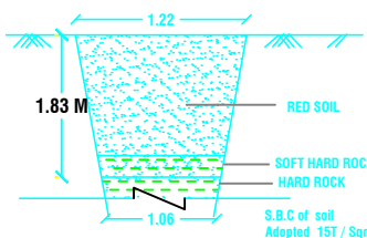
TRIAL PIT DETAILS
