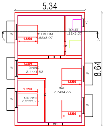
PRO.GROUND FLOOR PLAN
