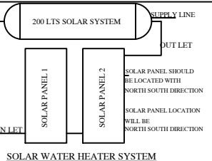
SOLAR WATER HEATER SYSTEM
