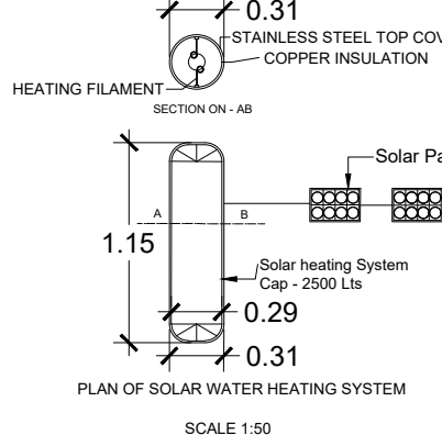
PLAN OF SOLAR WATER HEATING SYSTEM SCALE 1:30
