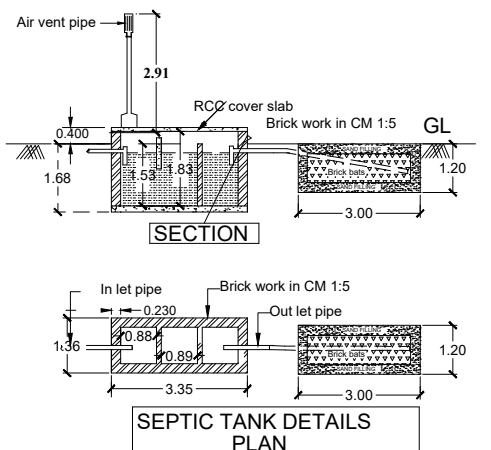
SEPTIC TANK DETAILS PLAN
