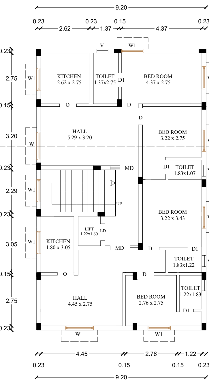
TYPICAL SECOND & THIRD FLOOR PLAN
