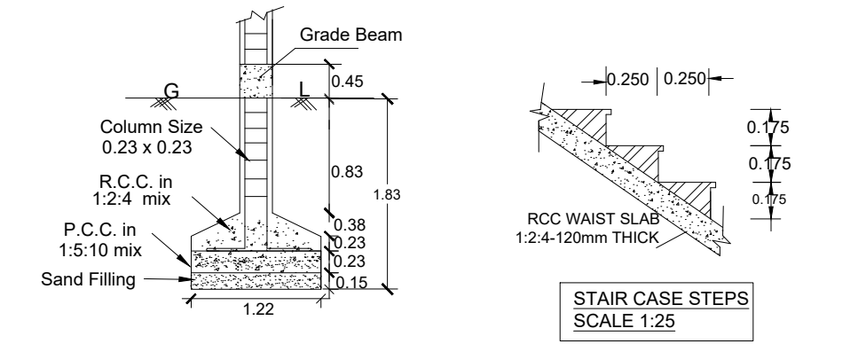
COLUMN DETAILS NOT TO SCALE
