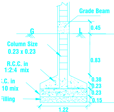
COLUMN DETAILS
