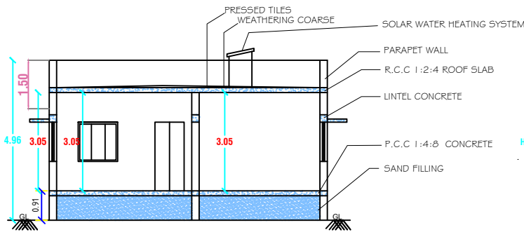
SECTION AT A-A
