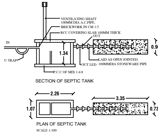
PLAN OF SEPTIC TANK SCALE 1:100
