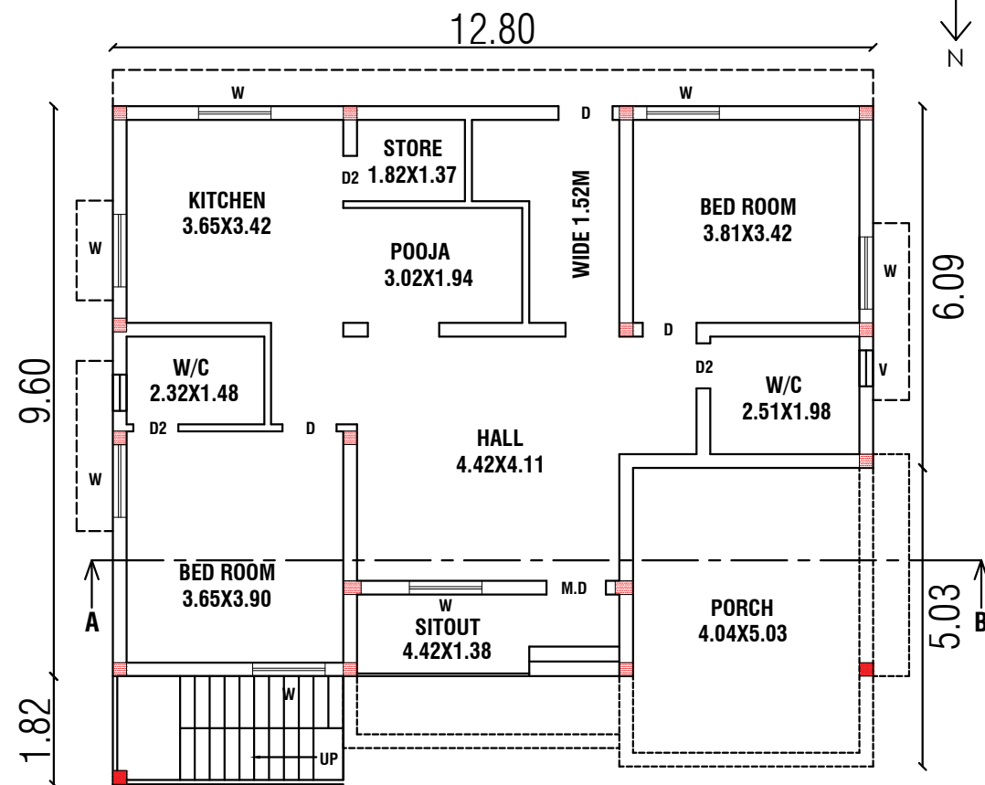
EXISTING & PROPOSED GROUND FLOOR PLAN
