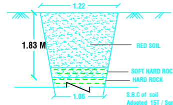
TRIAL PIT DETAILS
