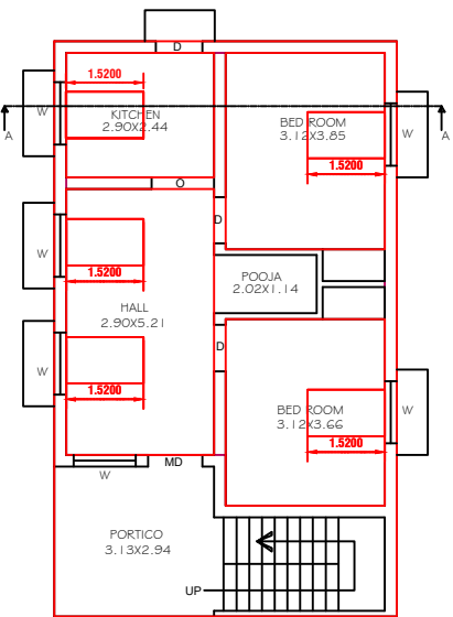
FLOOR PLAN
