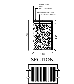
RAIN WATER HARVESTING PERCOLATION BED
