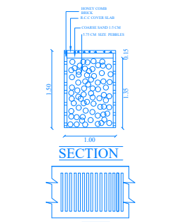
RAIN WATER HARVESTING PERCOLATION BED
