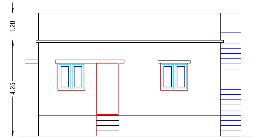
FRONT ELEVATION (PROPOSED)
