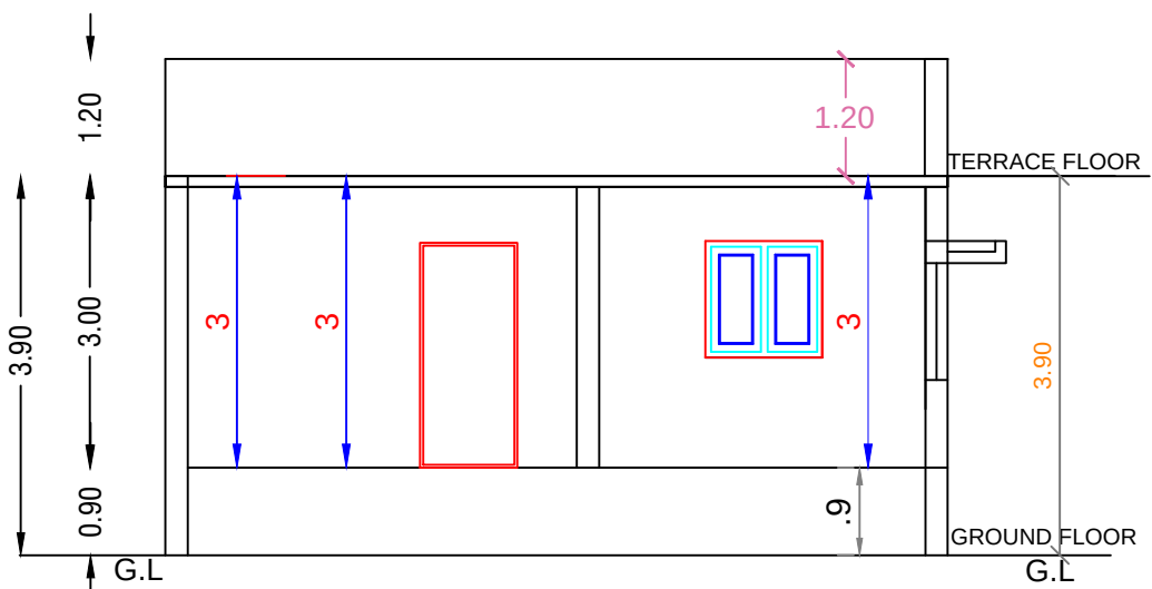
SECTION 'A-B' (PROPOSED)
