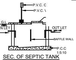
SEC. OF SEPTIC TANK
