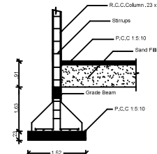
COLUMN DETAIL
