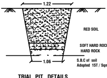
TRIAL PIT DETAILS NOT TO SCALE
