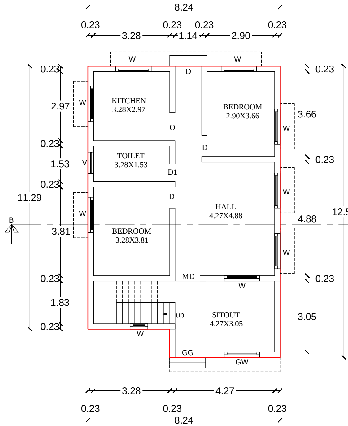
PRO- GROUND FLOOR PLAN
