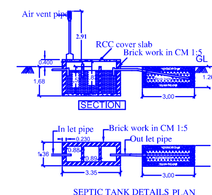
SEPTIC TANK DETAILS PLAN SCALE 1 : 200
