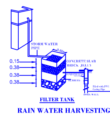
RAIN WATER HARVESTING SCALE 1 : 100
