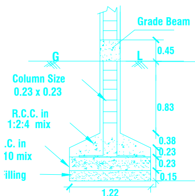
COLUMN DETAILS
