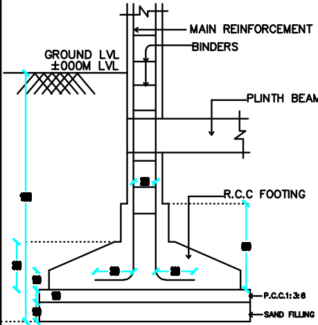
TYPICAL SECTION OF R.C.C COLUMN FOUNDATION SCALE : 1" = 2'-0" NOT TO SCALE
