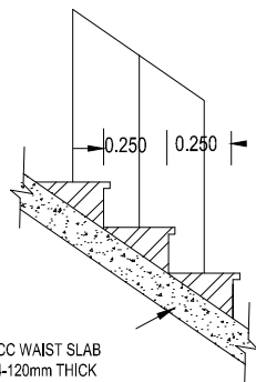
STAIR CASE DETAILS NOT TO SCALE
