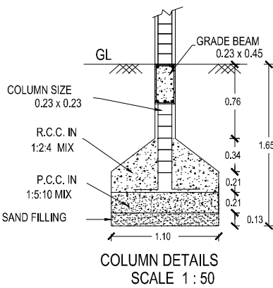
COLUMN DETAILS SCALE 1 : 50
