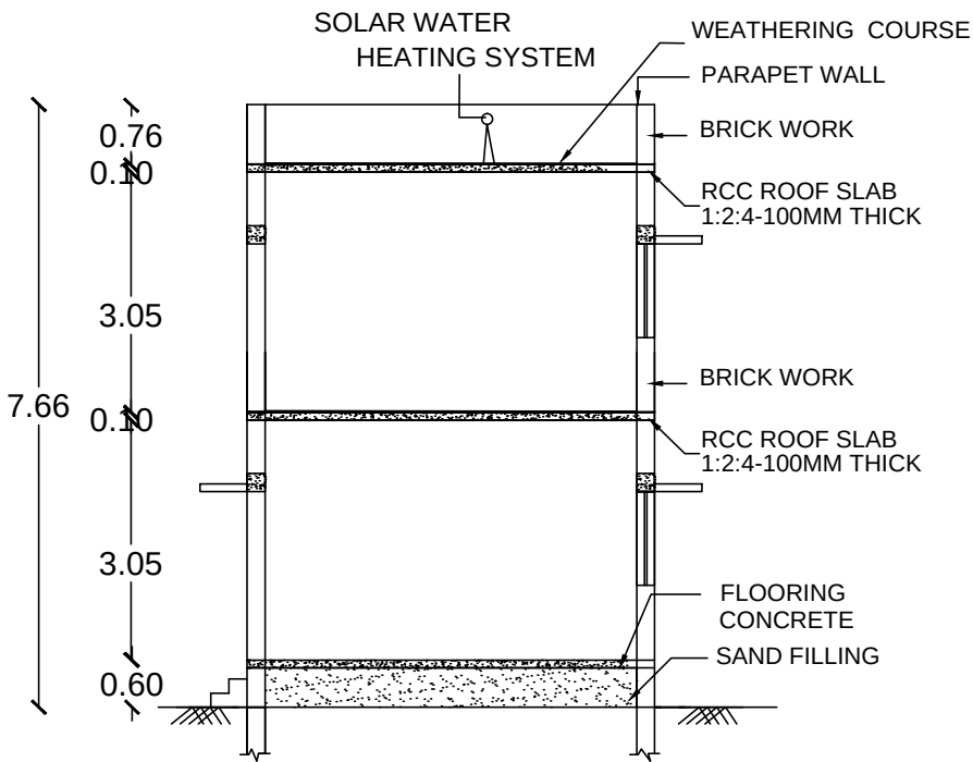
SECTION ON RM
