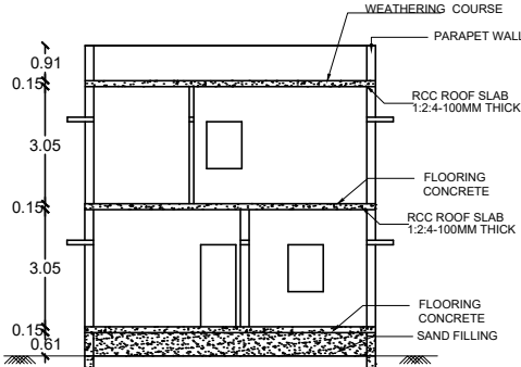
SECTION NP
