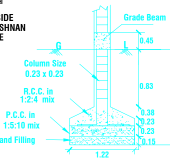
COLUMN DETAILS
