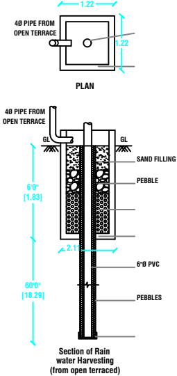
Section of Rain water Harvesting (from open terraced)
