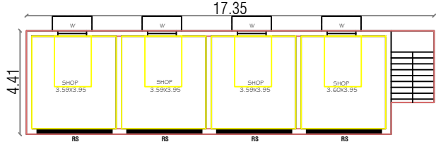
PRO.GROUND FLOOR PLAN
